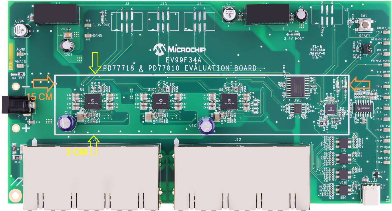
Figure 3. EV99F34A Dimension
