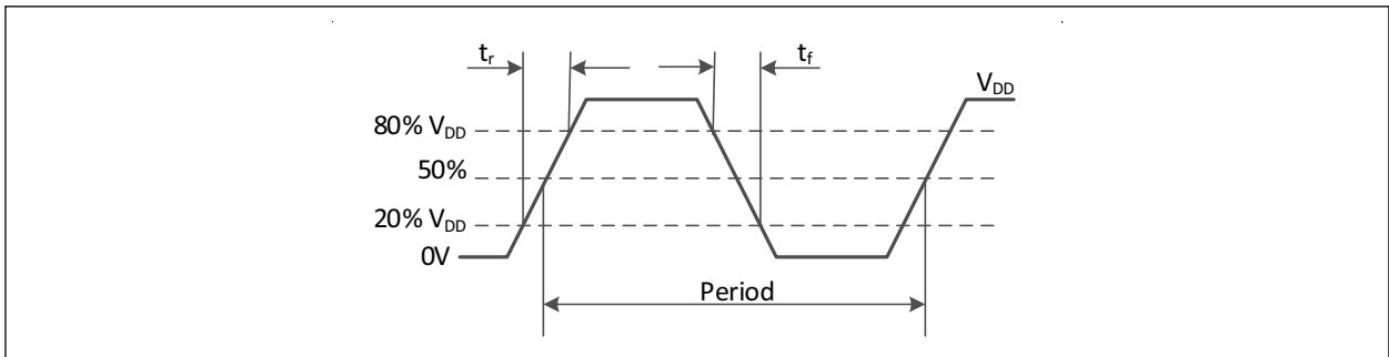
FIGURE 4-1: Output Waveform.
