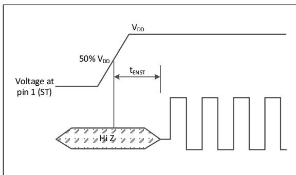
FIGURE 6-2: Enable Time with Pin 1 Configured as Standby (STB).
