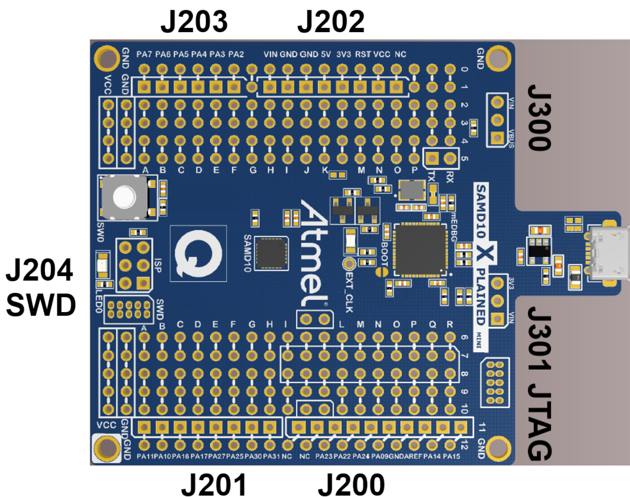
Figure 2-1. ATSAMD10-XMINI Overview
