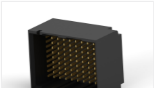
TE Part # 2007790-1 IMP100S,H,V3P10C,UG,DEW39,4.5
