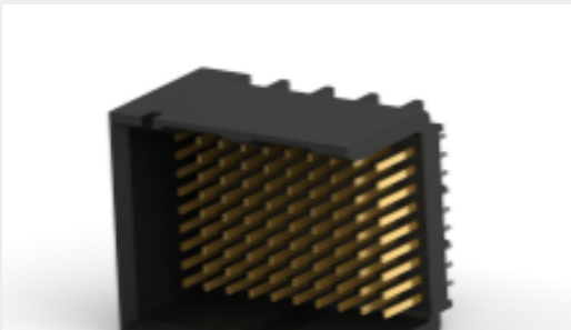
TE Part # 2007789-1 IMP100S,H,V3P10C,UG,LEW39,4.5
