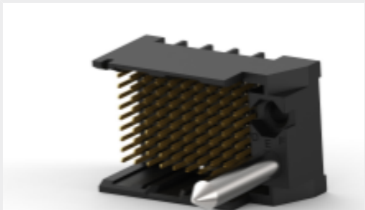
TE Part # 2007781-1 IMP100S,H,V3P10C,RG,OEW39,4.5
