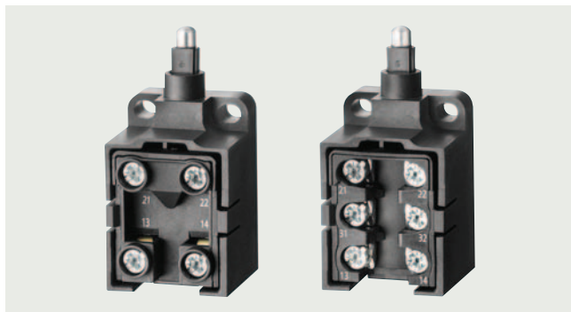
Open-type design
