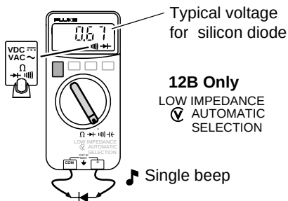
Forward Bias
