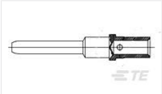
TE Part #208271-3 PIN CONT, SZ 12
