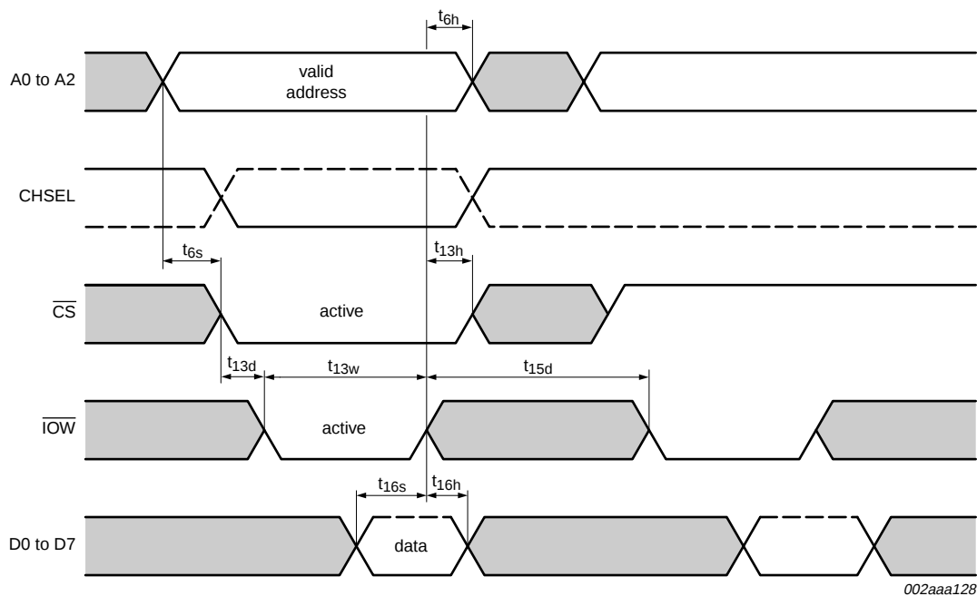
Fig 5. General write timing
