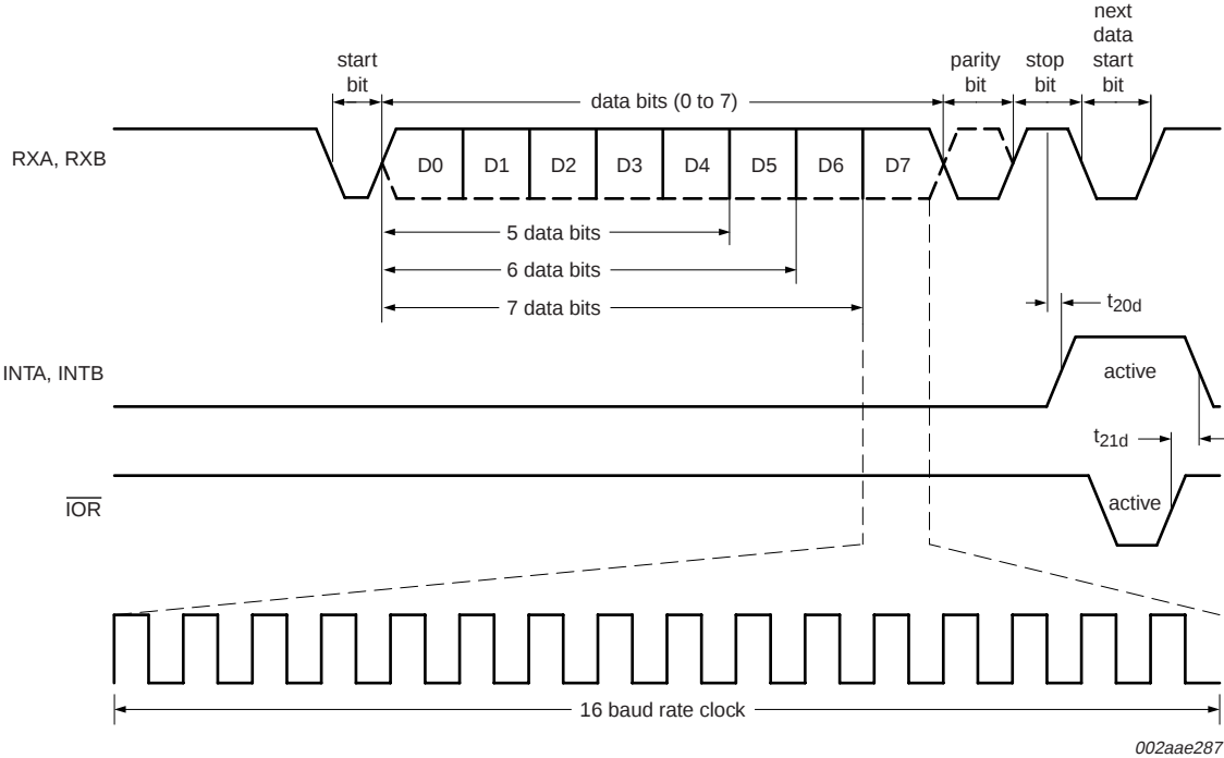
Fig 9. Receive timing
