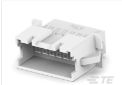
TE Part # 1-2324584-4 HSG,REC,PANEL MOUNT,DUALROW,EP2.5
