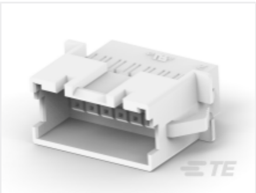
TE Part # 1-2323745-4 HSG,REC,PANEL MOUNT,GWT,DUALROW,EP2.5
