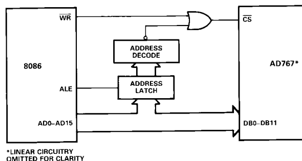
Figure 7. 8086 – AD767 Interface
