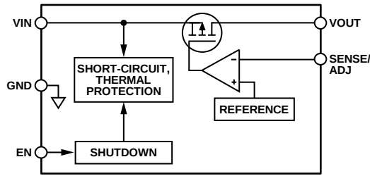
Figure 42. Internal Block Diagram
