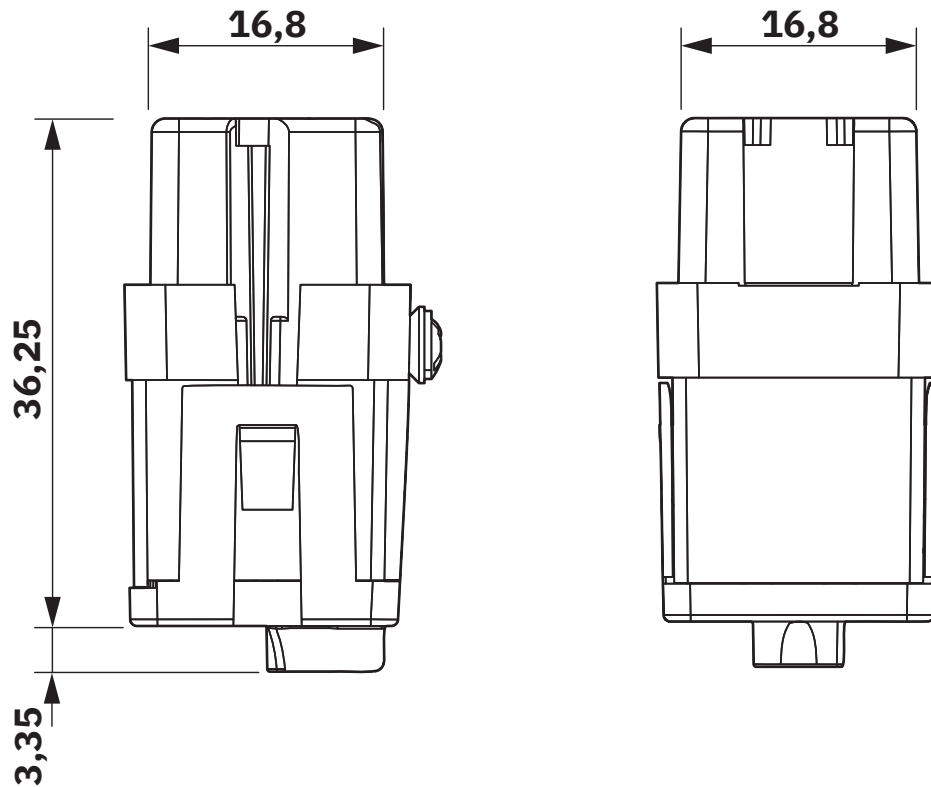
Dimensional drawing
