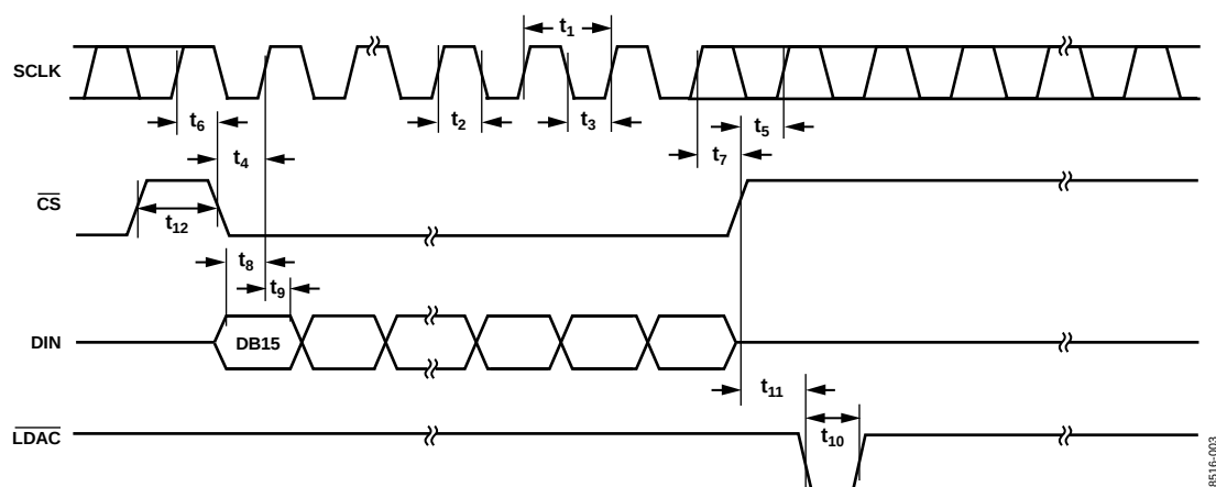
Figure 3. Timing Diagram
