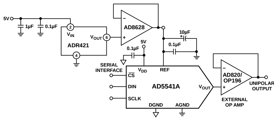
Figure 31. Unipolar Output
