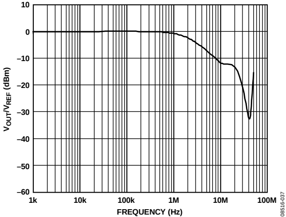
Figure 29. Multiplying Bandwidth
