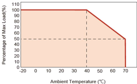
1. Derating Curve
