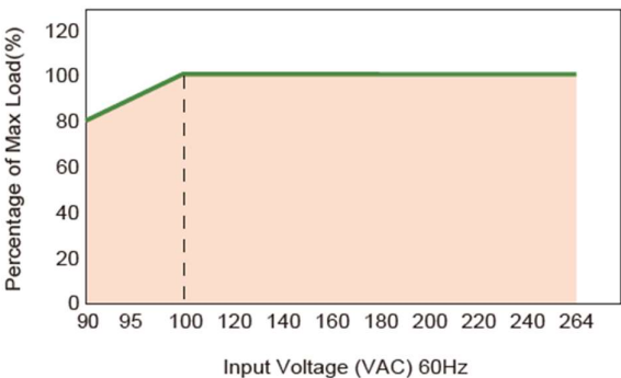
2. Static Characteristics
