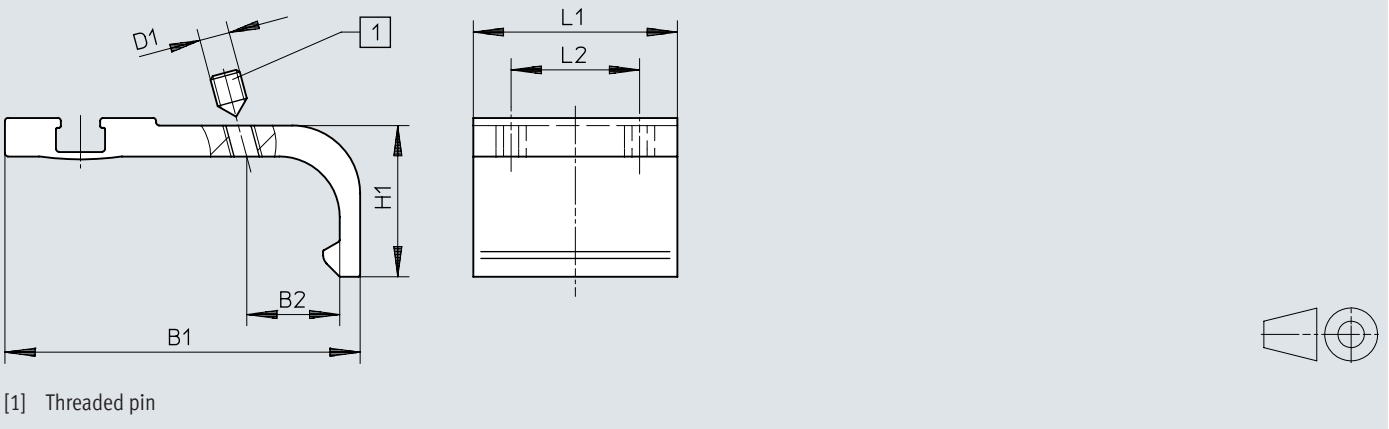
Dimensions – Mounting kit SMB-8-FENG
