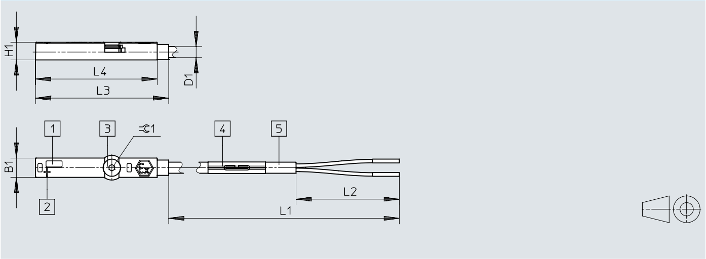
Dimensions – Proximity switch open end
