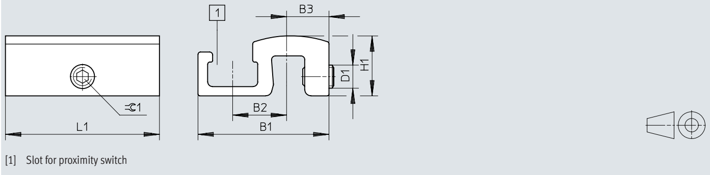
Dimensions – Mounting kit SMB-8-C
