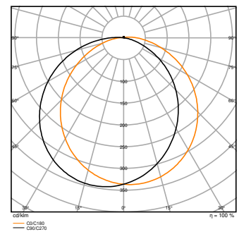
BLKH CBO RD EYELID V 16W 857
