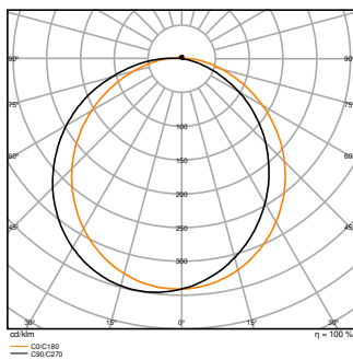
BLKH CBO RD EYELID V 16W 830
