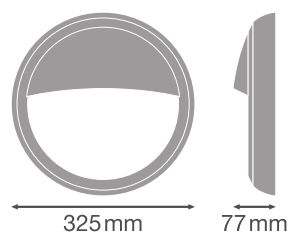
BLKH CBO RD EYELID 325 WT
