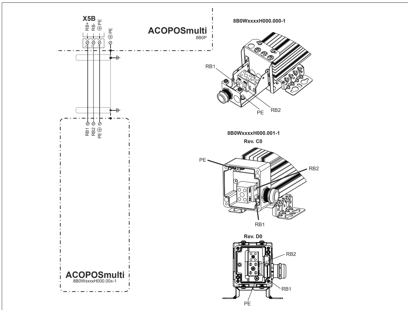
Figure 2: 8B0W - Pinout overview
