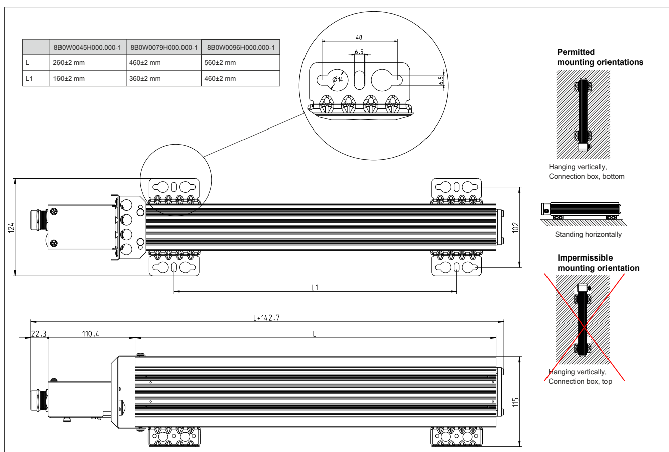
Figure 1: Dimension diagram and installation dimensions
