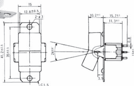
(ロッカー取付例) (Mount with Rocker)
