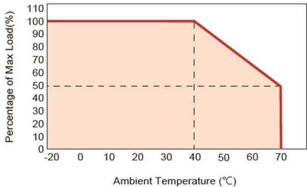
1. Derating Curve
