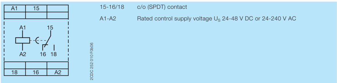
Connection diagram
