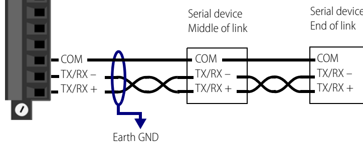
RS-485 2-Wire
