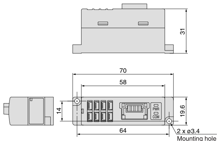
EX510-S□01B
