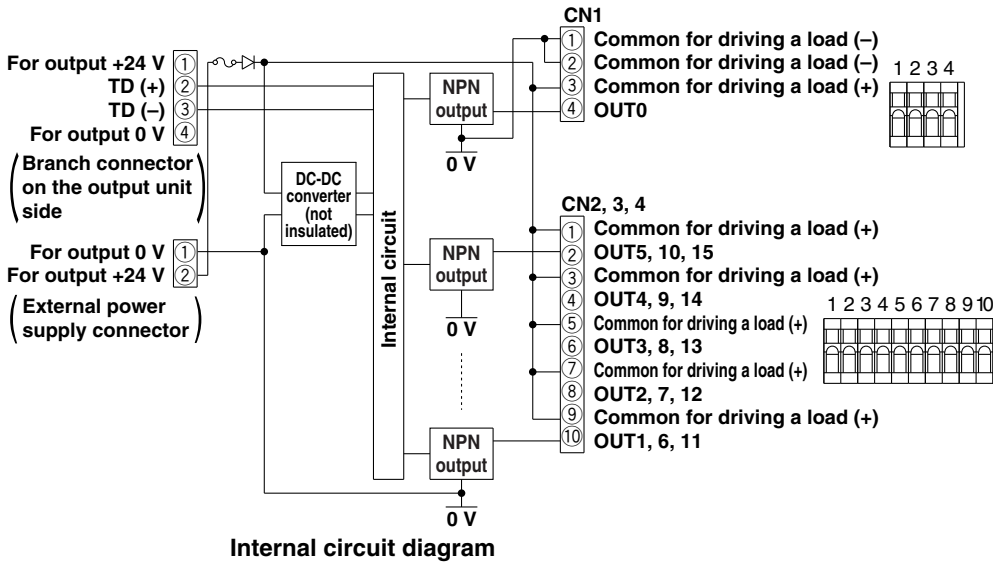
Internal circuit diagram
