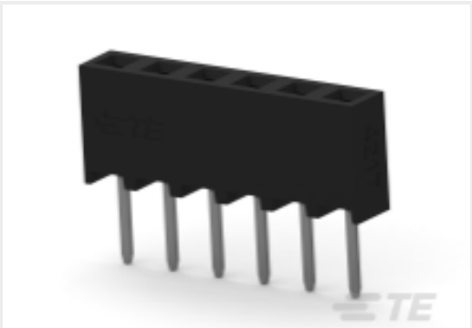
TE Part #2314876-6 6P,2MM,B-B,REC,SRVT,2.7,0.1AU,TB
