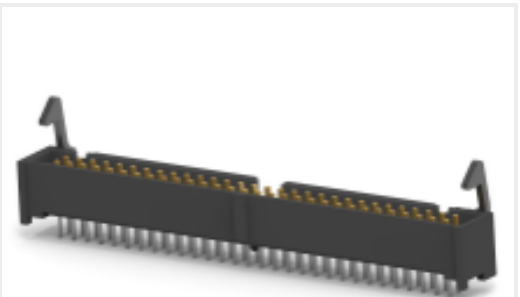
TE Part # 1-1761608-6 IDC LOW PRO HDR 60P VERT SHT LAT BLK
