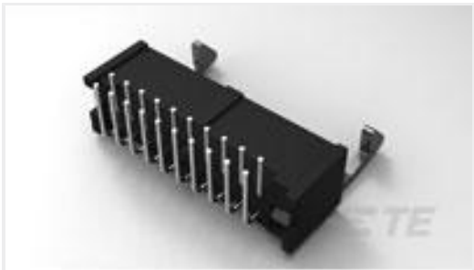
TE Part # 3-1761607-6 IDC LOW PRO HDR 60P RA LAT
