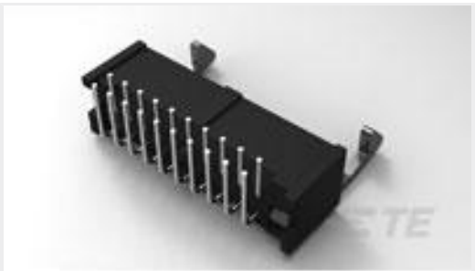
TE Part # 1-1761607-6 IDC LOW PRO HDR 60P RA LAT
