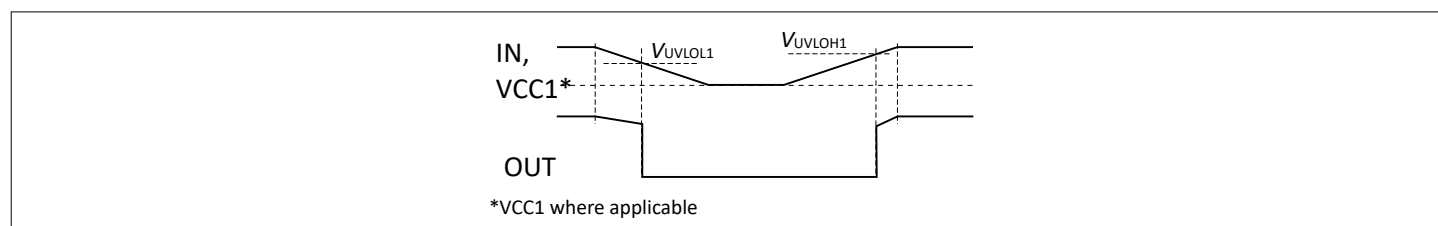
Figure 8 UVLO behavior
