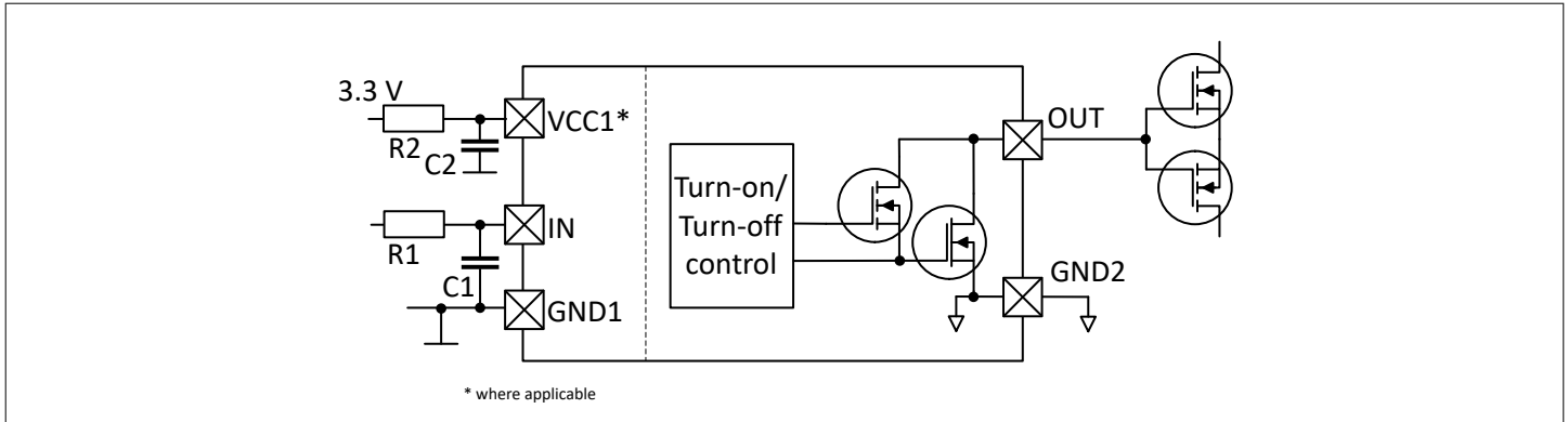
Figure 16 Fast turn-off
