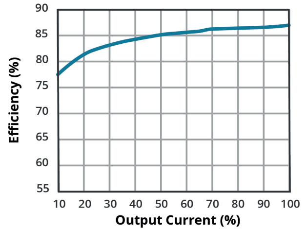
EFFICIENCY VS OUTPUT LOAD AE40-EW-S24
