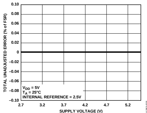
Figure 22. Total Unadjusted Error vs. Supply Voltage, Gain = 1
