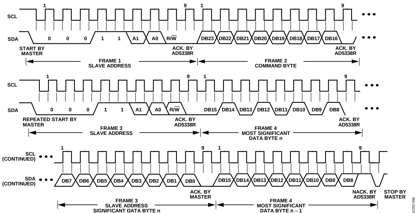
Figure 45. I²C Read Operation
