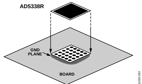
Figure 52. Paddle Connection to Board
