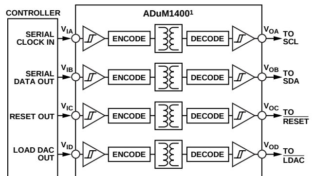
Figure 53. Isolated Interface
