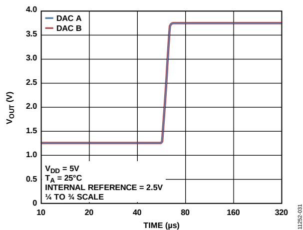
Figure 30. Settling Time
