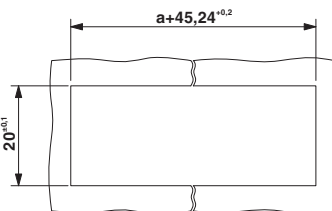
Dimensioned drawing
