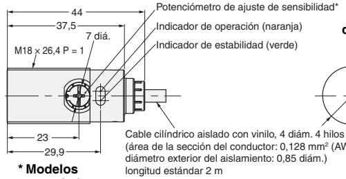
Vista frontal
