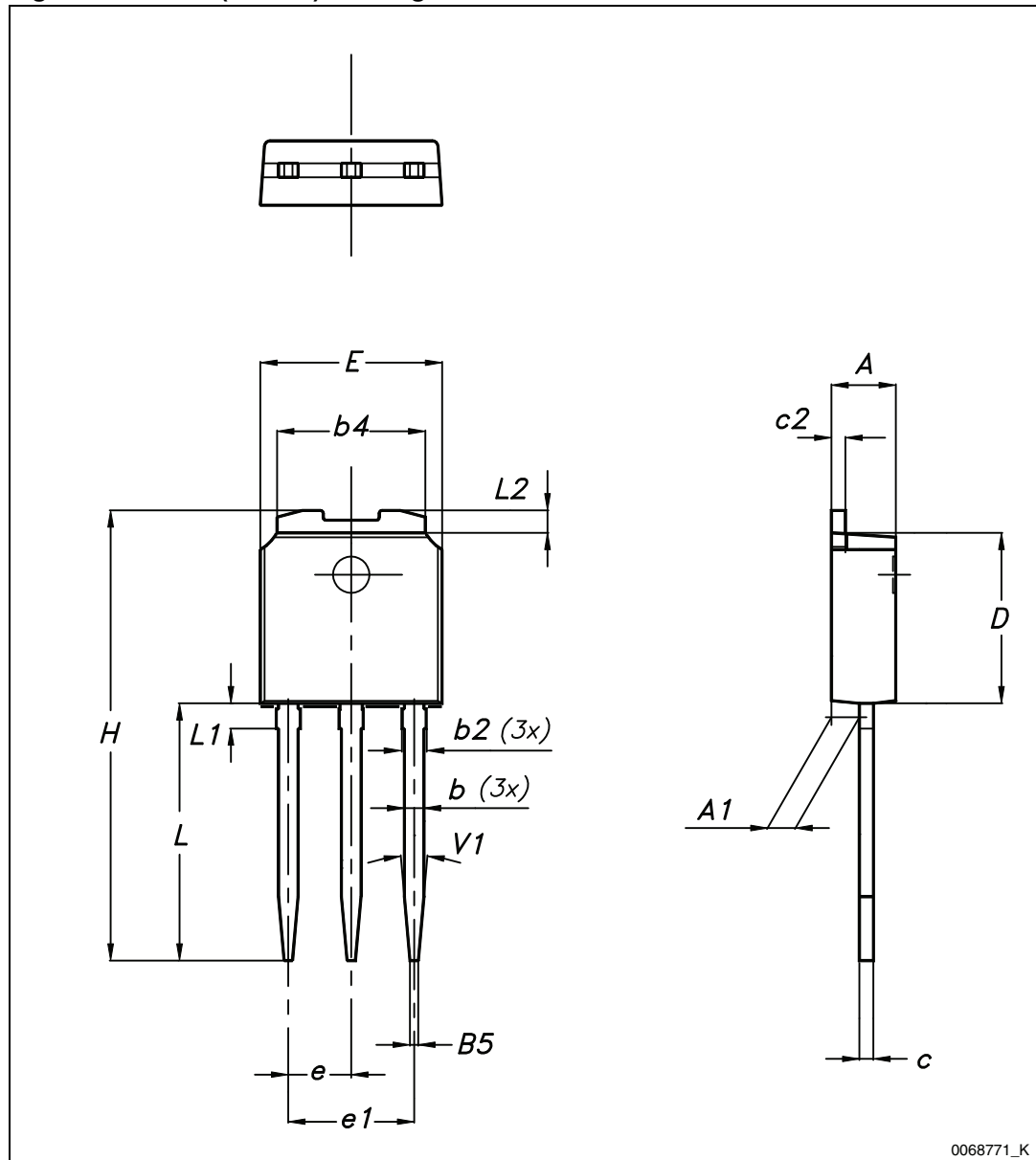
Figure 11. IPAK (TO-251) drawing
