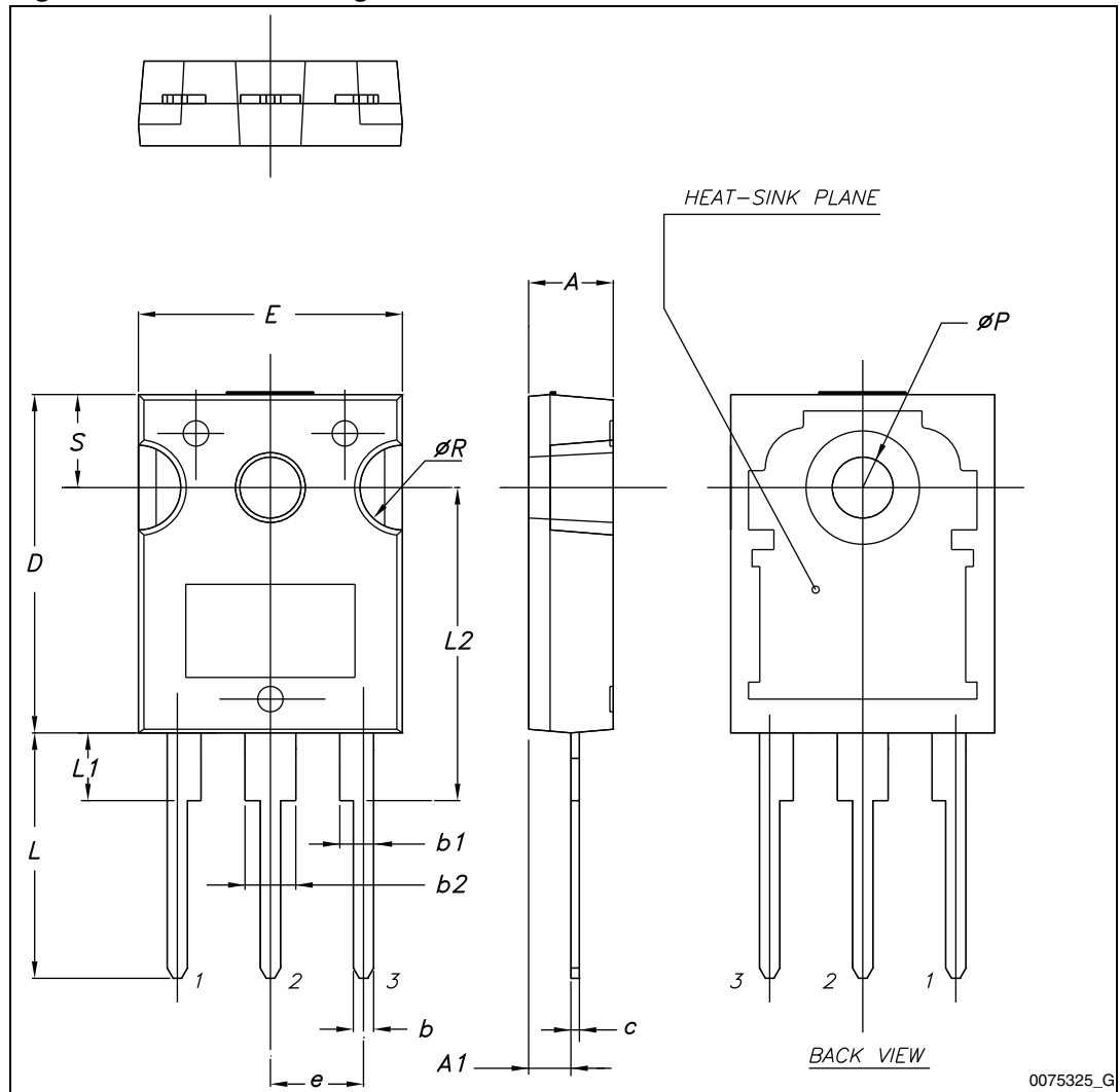
Figure 12. TO-247 drawing
