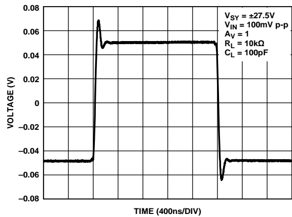
Figure 40. Small Signal Transient Response, V_{SY} = \pm 27.5V
