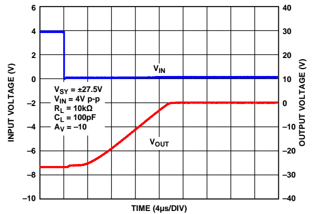
Figure 58. Negative Overload Recovery, V_{SY} = \pm 27.5V
