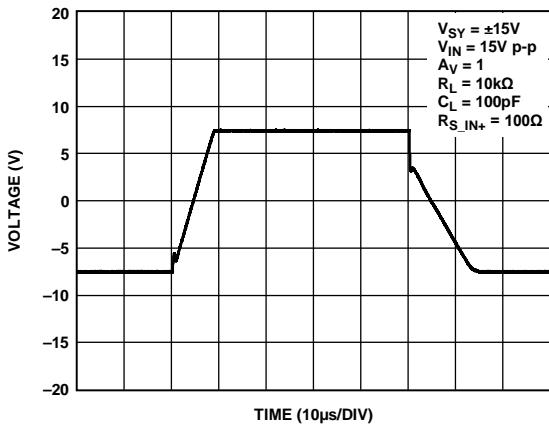
Figure 36. Large Signal Transient Response, V_{SY} = \pm 15V
