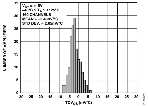
Figure 9. Input Offset Voltage Drift Distribution, V_{SY} = \pm 15\text{V}
