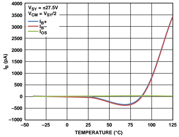
Figure 20. Input Bias Current ( I_B ) vs. Temperature, V_{SY} = \pm 27.5V
