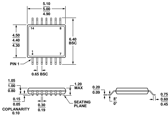
Figure 90. 14-Lead Thin Shrink Small Outline Package [TSSOP] (RU-14)
