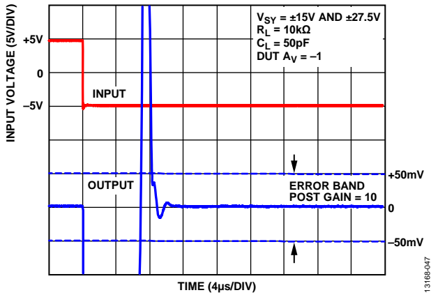
Figure 66. Negative Settling Time to 0.1%, V_{SY} = \pm 15 V and \pm 27.5 V
