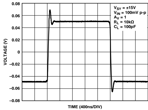
Figure 39. Small Signal Transient Response, V_{SY} = \pm 15V
