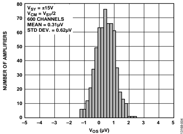
Figure 6. Input Offset Voltage Distribution, V_{SY} = \pm 15\text{V}
