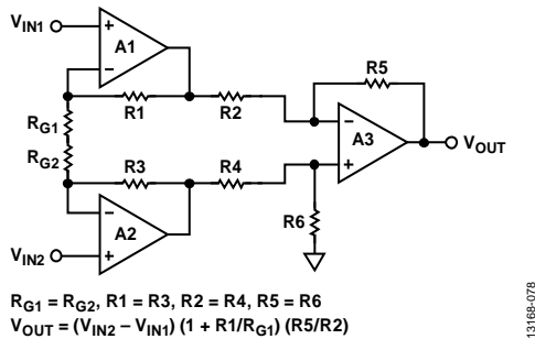
Figure 80. Discrete 3-Op Amp Instrumentation Amplifier
