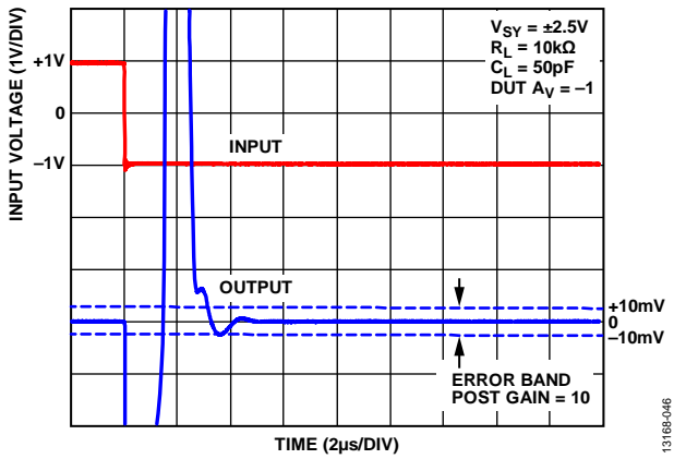
Figure 65. Negative Settling Time to 0.1%, V_{SY} = \pm 2.5 V
