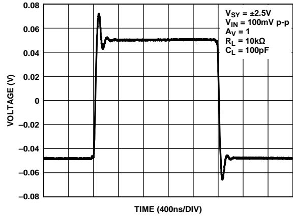
Figure 38. Small Signal Transient Response, V_{SY} = \pm 2.5V
