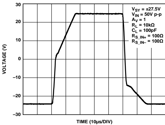
Figure 37. Large Signal Transient Response, V_{SY} = \pm 27.5V
