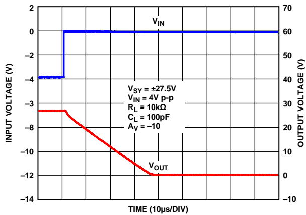
Figure 55. Positive Overload Recovery, V_{SY} = \pm 27.5V
