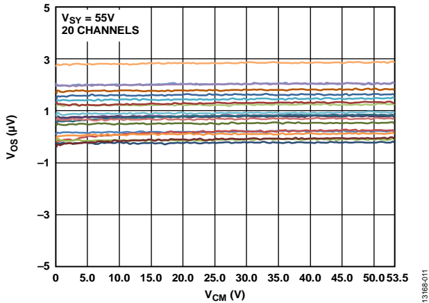
Figure 13. Input Offset Voltage ( V_{OS} ) vs. Common-Mode Voltage ( V_{CM} ), V_{SY} = 55V
