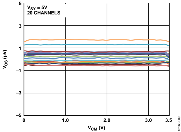
Figure 11. Input Offset Voltage ( V_{OS} ) vs. Common-Mode Voltage ( V_{CM} ), V_{SY} = 5V
