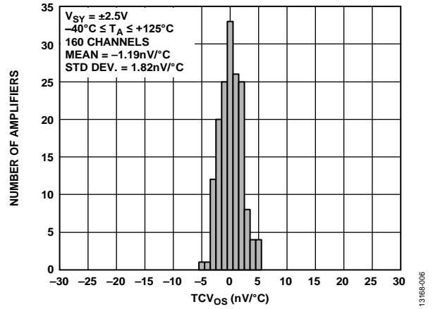
Figure 8. Input Offset Voltage Drift Distribution, V_{SY} = \pm 2.5\text{V}
