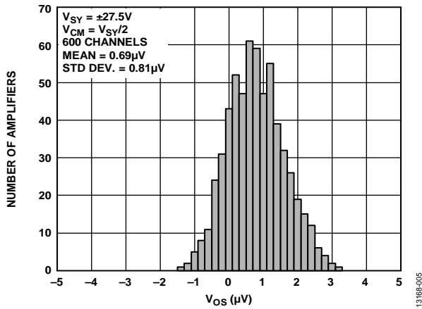
Figure 7. Input Offset Voltage Distribution, V_{SY} = \pm 27.5\text{V}
