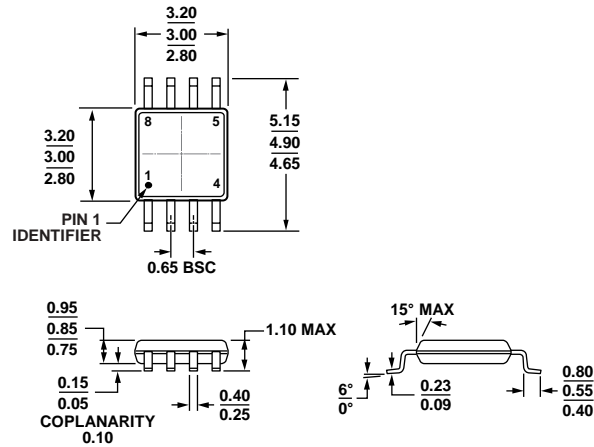
Figure 87. 8-Lead Mini Small Outline Package [MSOP] (RM-8)
