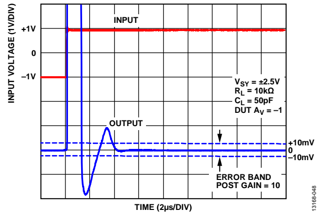
Figure 68. Positive Settling Time to 0.1%, V_{SY} = \pm 2.5 V
