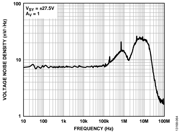
Figure 61. Voltage Noise Density vs. Frequency, V_{SY} = \pm 27.5V
