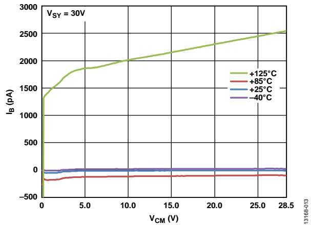
Figure 15. Input Bias Current ( I_B ) vs. Common-Mode Voltage ( V_{CM} ), V_{SY} = 30V
