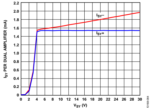
Figure 86. Supply Current ( I_{SY} ) per Dual Amplifier vs. Supply Voltage ( V_{SY} ) (ADA4522-2/ADA4522-4 as a Comparator)
