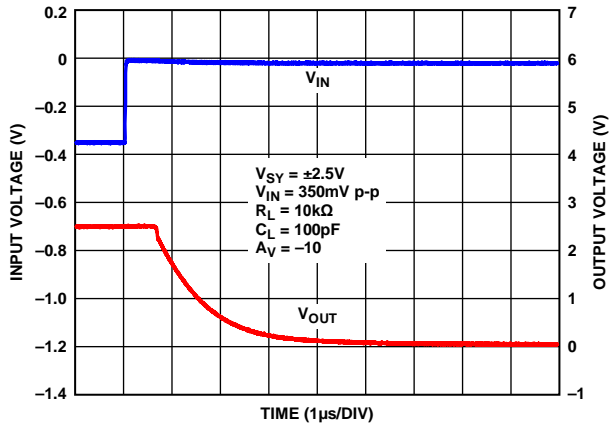
Figure 53. Positive Overload Recovery, V_{SY} = \pm 2.5V
