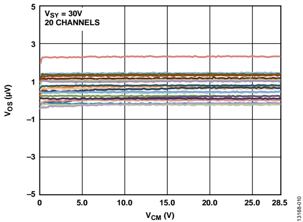
Figure 12. Input Offset Voltage ( V_{OS} ) vs. Common-Mode Voltage ( V_{CM} ), V_{SY} = 30V
