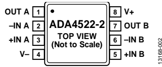
Figure 3. ADA4522-2 Pin Configuration
