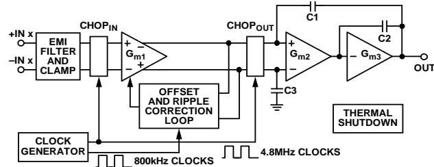
Figure 70. ADA4522-2/ADA4522-4 Block Diagram
