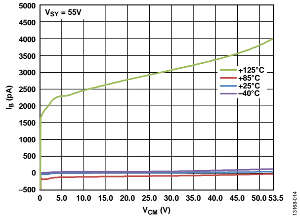
Figure 16. Input Bias Current ( I_B ) vs. Common-Mode Voltage ( V_{CM} ), V_{SY} = 55V
