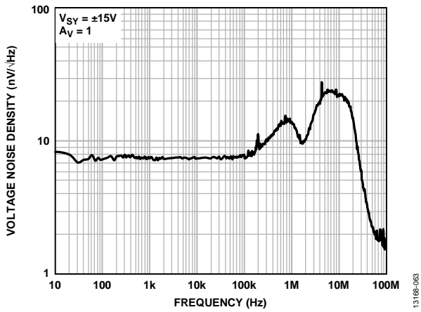
Figure 60. Voltage Noise Density vs. Frequency, V_{SY} = \pm 15V
