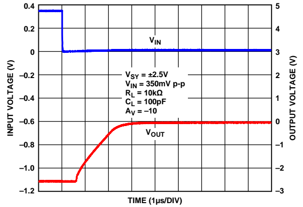
Figure 56. Negative Overload Recovery, V_{SY} = \pm 2.5V
