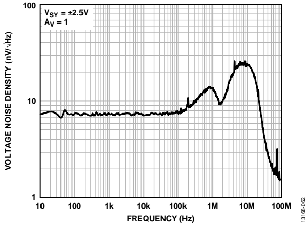
Figure 59. Voltage Noise Density vs. Frequency, V_{SY} = \pm 2.5V
