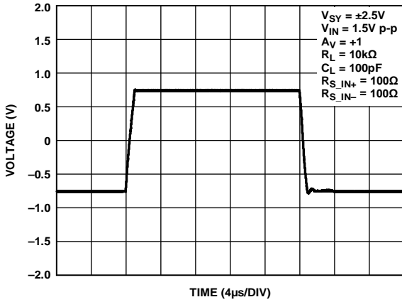
Figure 35. Large Signal Transient Response, V_{SY} = \pm 2.5V
