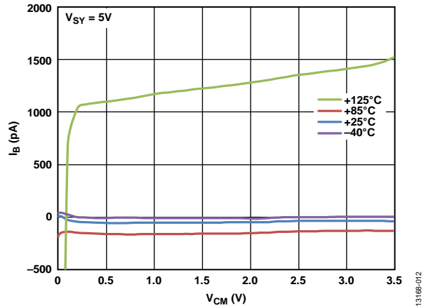
Figure 14. Input Bias Current ( I_B ) vs. Common-Mode Voltage ( V_{CM} ), V_{SY} = 5V
