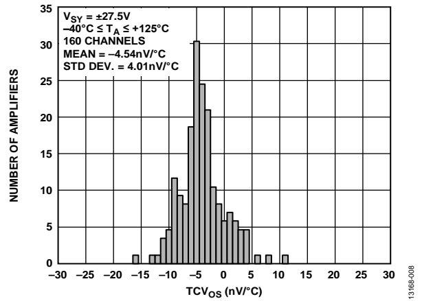
Figure 10. Input Offset Voltage Drift Distribution, V_{SY} = \pm 27.5\text{V}
