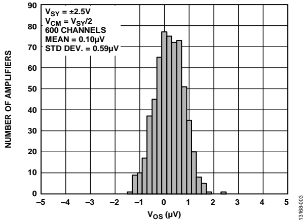
Figure 5. Input Offset Voltage Distribution, V_{SY} = \pm 2.5\text{V}
