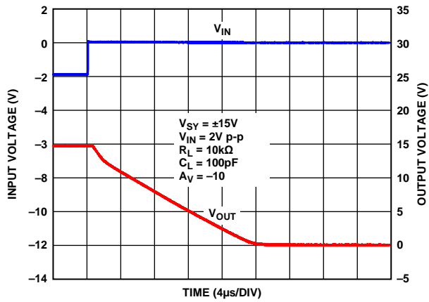
Figure 54. Positive Overload Recovery, V_{SY} = \pm 15V
