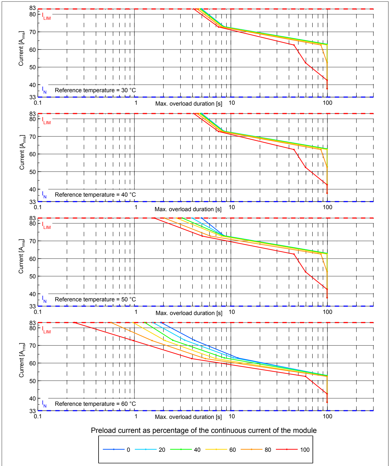
Figure 2: 8BVI0330HCSx.000-x - Overload characteristics, overload response - ERROR+STOP
