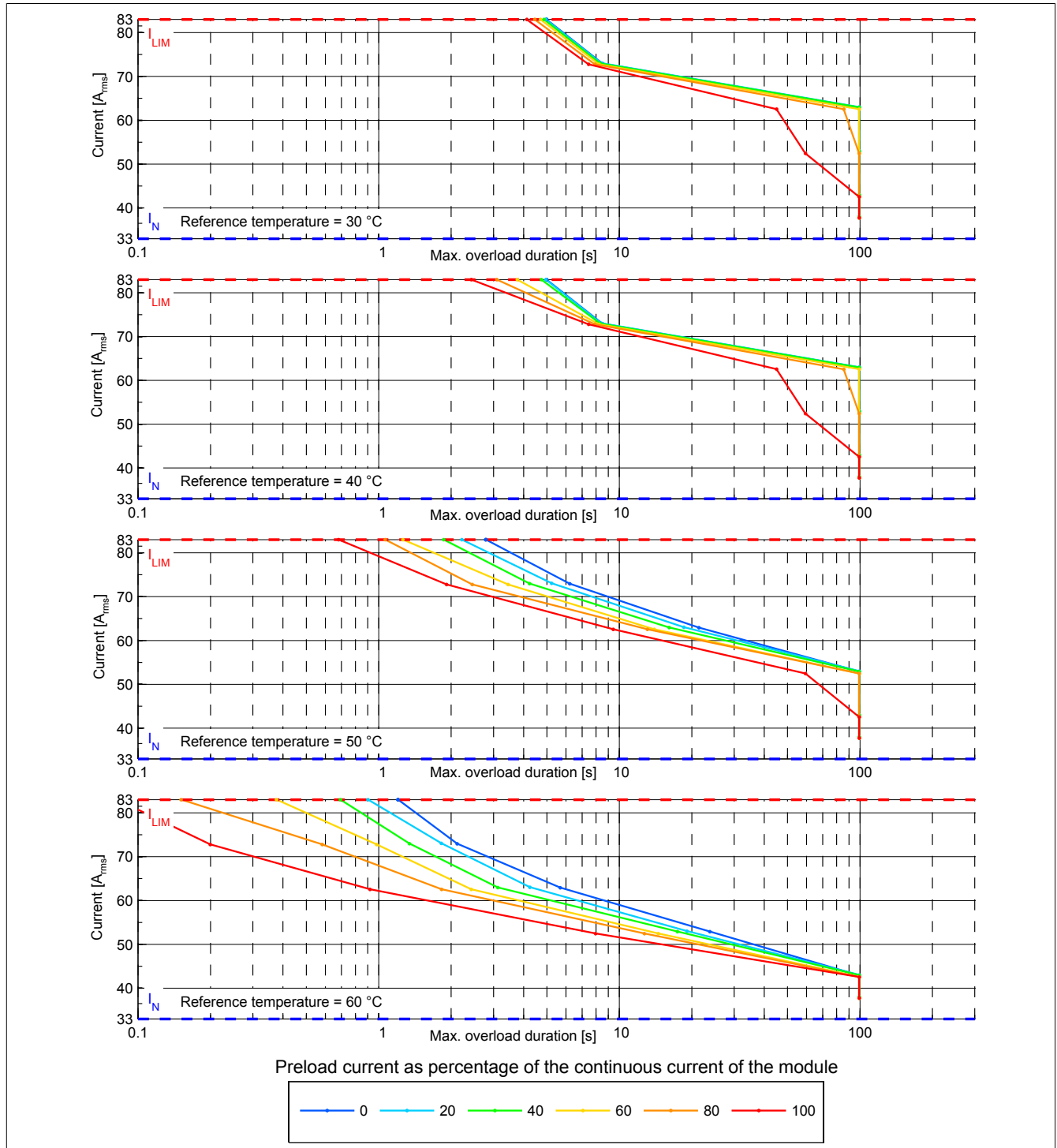
Figure 1: 8BVI0330HCSS.000-x - Overload characteristics, overload response - WARNING
