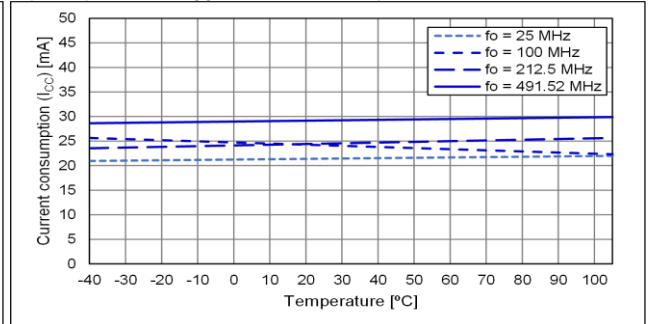
Output option:A, V CC = 3.63 V, Temp. Characteristic
