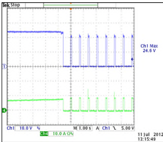
24V OUT, 90VAC
