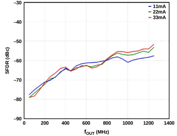
Figure 72. SFDR vs. f_{OUT} over DAC I_{OUTFS}
