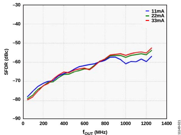
Figure 18. SFDR vs. f_{OUT} over DAC I_{OUTS}
