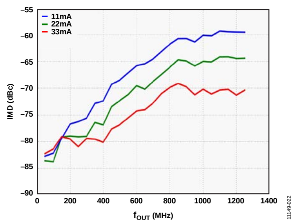
Figure 19. IMD vs. f_{OUT} over DAC I_{OUTS}
