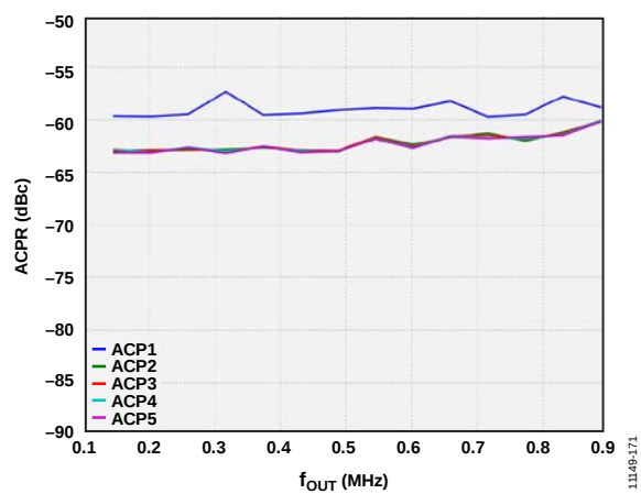
Figure 54. 32-Carrier ACPR vs. f_{OUT}
