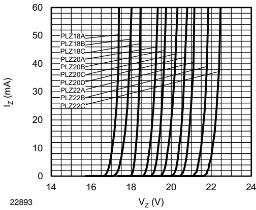
Fig. 9 - Breakdown Characteristics
