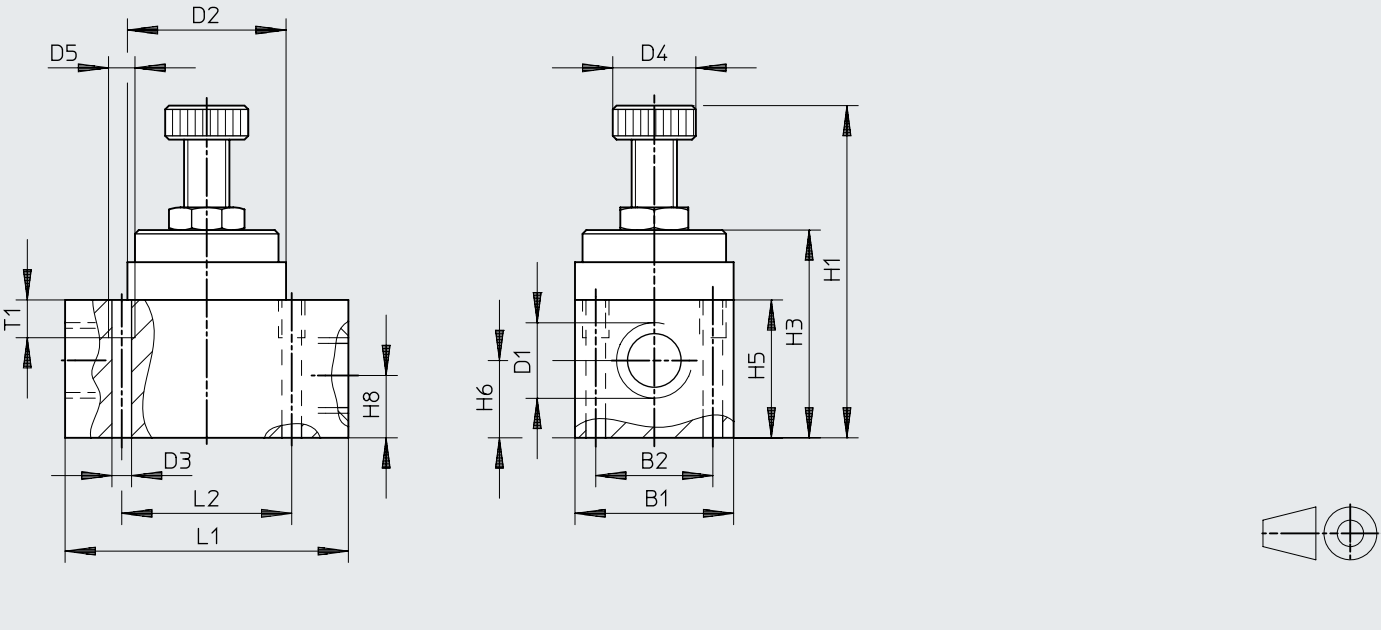
Dimensions – GR-1/2
