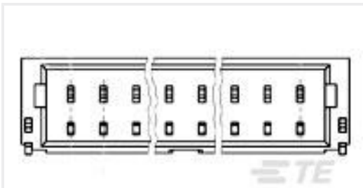
TE Part #1-1734709-5 1.0 WTB HDR SR RA 15 POS
