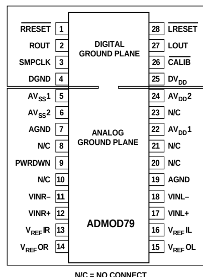
Figure 5. ADM0D79 Recommended Ground Plane
