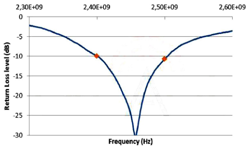
Return Loss
