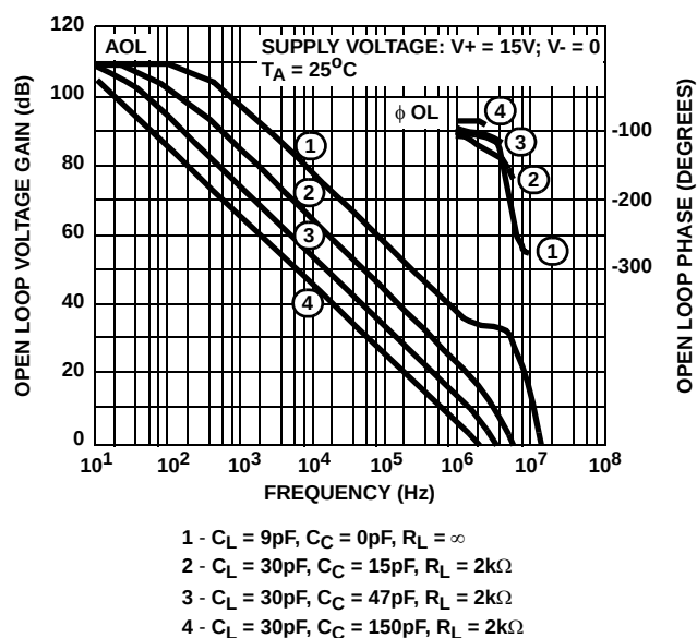
FIGURE 19. OPEN-LOOP RESPONSE
