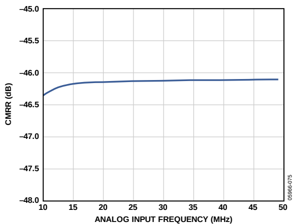
Figure 31. CMRR vs. Analog Input Frequency, f_{\text{SAMPLE}} = 100 \text{ MSPS}
