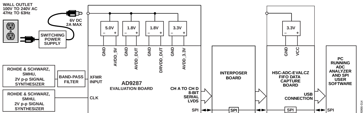
Figure 60. Evaluation Board Connection
