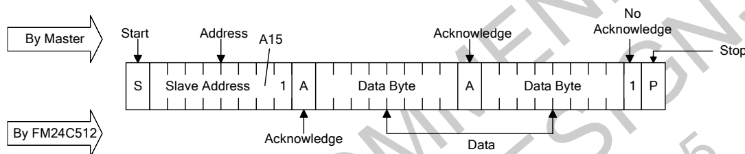
Figure 8. Sequential Read
