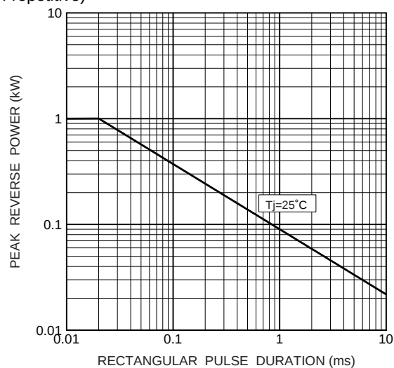
逆耐量特性（非繰り返し） Typical reverse power characteristics (Non-repetitive)
