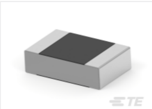
TE Part #5-2176264-9 RN 0805 4R75 0.1% 10PPM 1K RL
