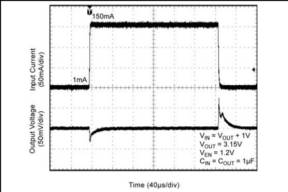
FIGURE 2-19: Load Transient ( V_{SEL} = \text{High} ).
