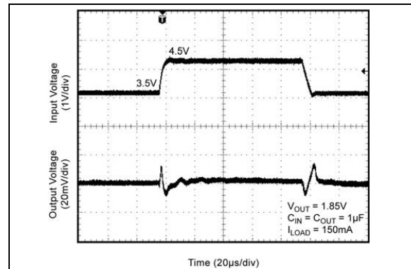
FIGURE 2-18: Line Transient ( V_{SEL} = \text{Low} ).
