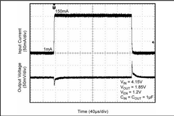
FIGURE 2-20: Load Transient ( V_{SEL} = \text{Low} ).
