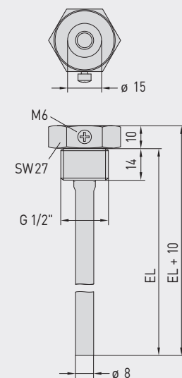
Dimensional drawing TH08-VA/xx [mm]
