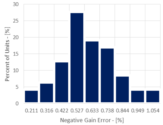
Negative Gain Error Histogram
