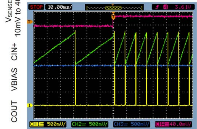
TS1108-20 Coulomb Counting V_{VBIAS}=1.5V , V_{CIN-}=2.5V
