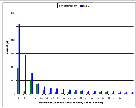
Figure 13 Harmonics in boost follower
