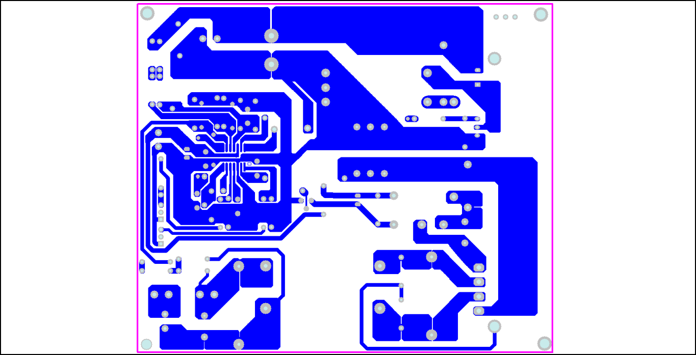
Figure 5 Bottom layer view
