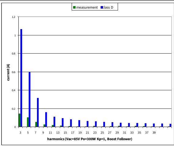
Figure 11 Harmonics in boost follower
