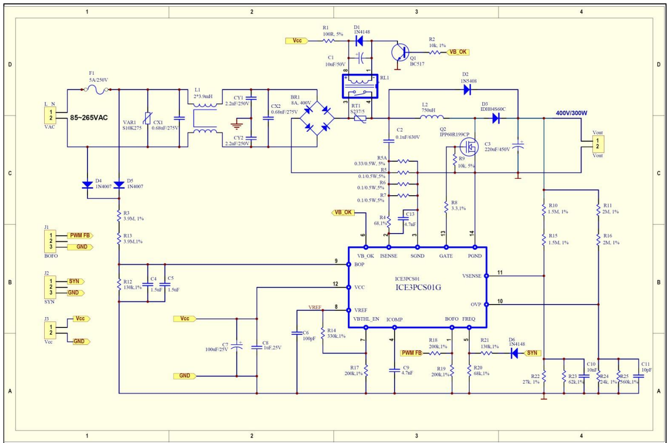
Figure 3 Schematic of 300 W PFC demo board
