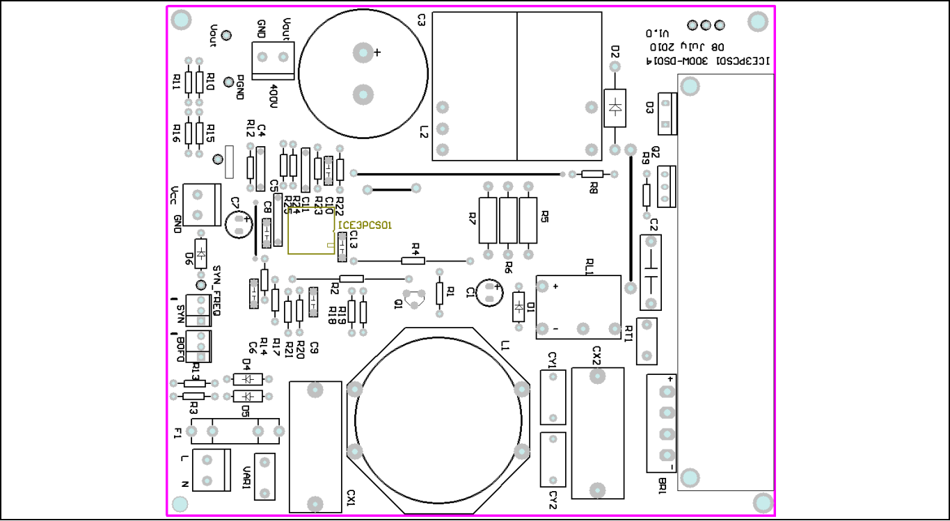
Figure 4 Top layer view
