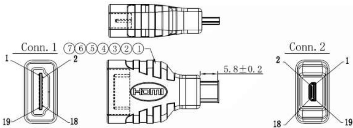
Pin Assignment
